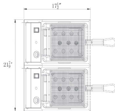
Basket Size: 8.8" W x 8.8" D x 6.8" H
