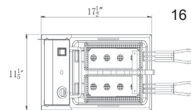
Basket Size: 4.5" W x 9.5" D x 4" H
