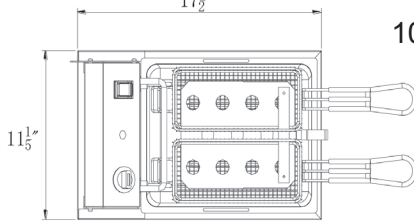
Basket Size: 4.5" W x 9.5" D x 6" H 17 1/2"
