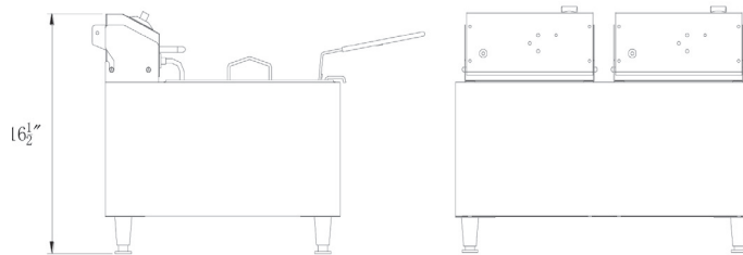
Basket Size: 8.8" W x 8.8" D x 6.8" H
